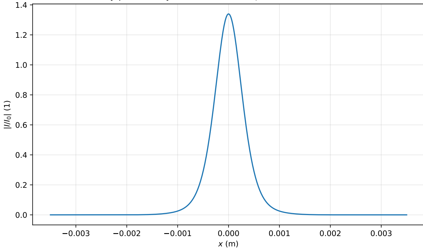
Intensity profile I(x, y = 0, z = 1.831m)/I_0 , P_{in}=0.8P_{cr} , artificial time
